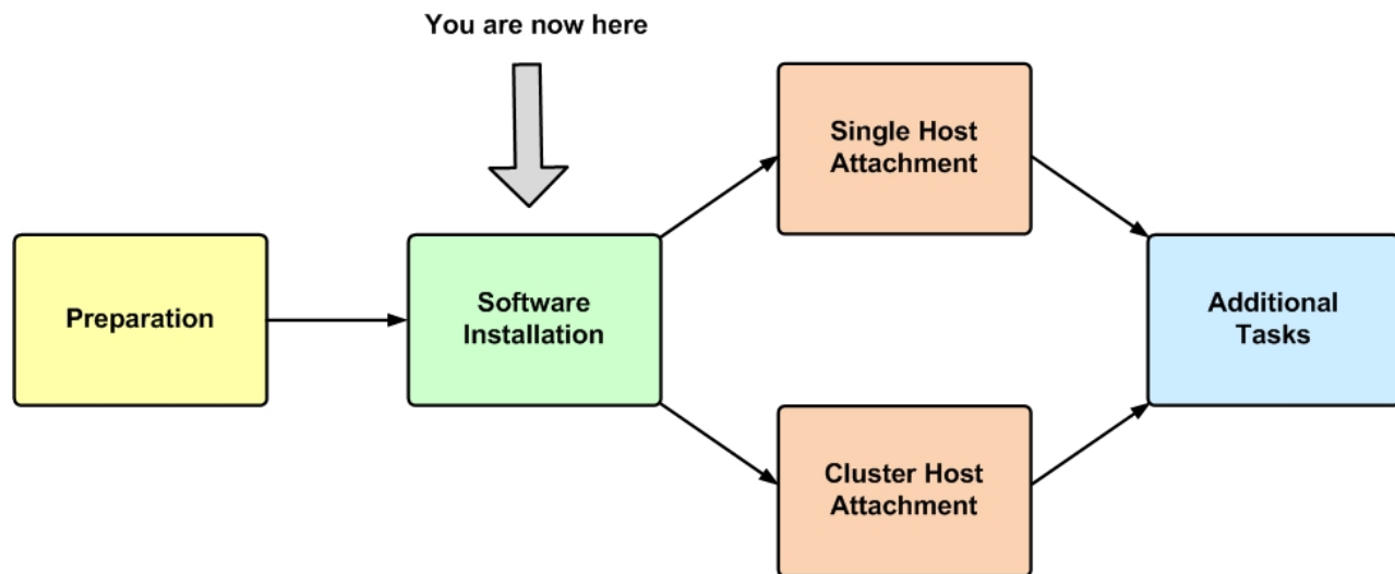
Figure 18. Software installation
