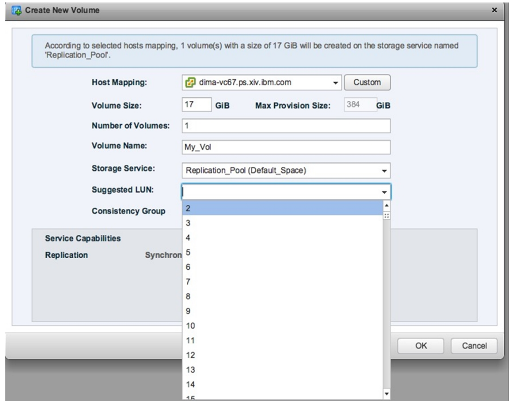
Figure 86. Selecting LUN
