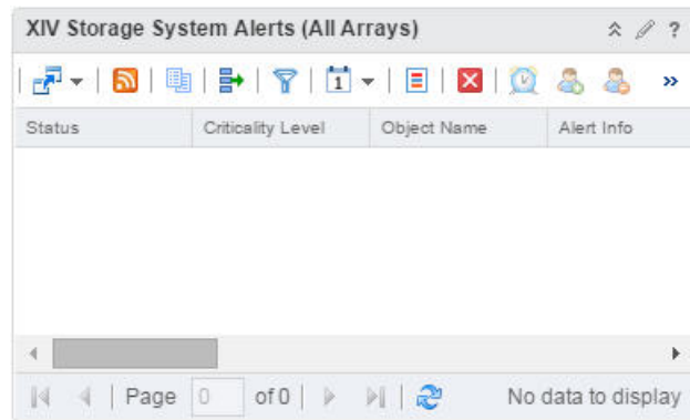
Figure 122. Alert widget
