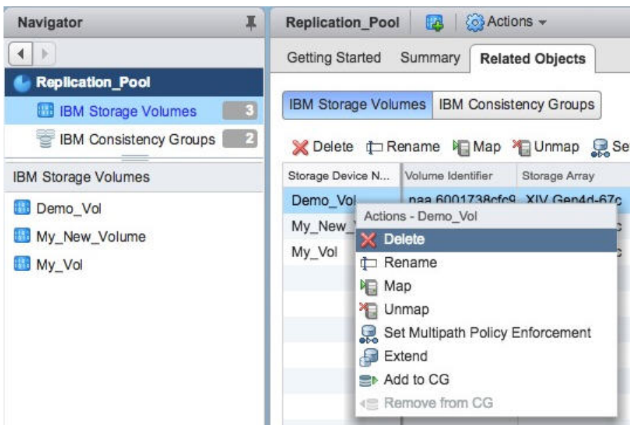
Figure 97. Delete volume
