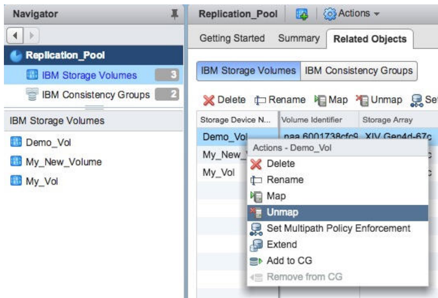
Figure 96. Unmap volume
