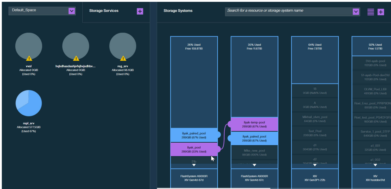
Figure 48. Paired pools
