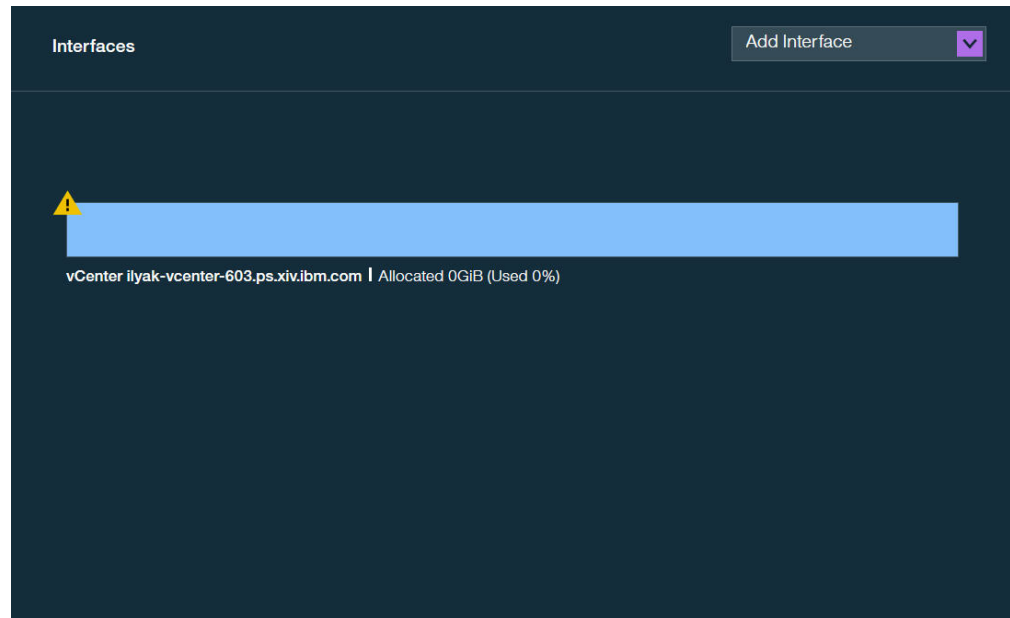
Figure 65. Interfaces pane
