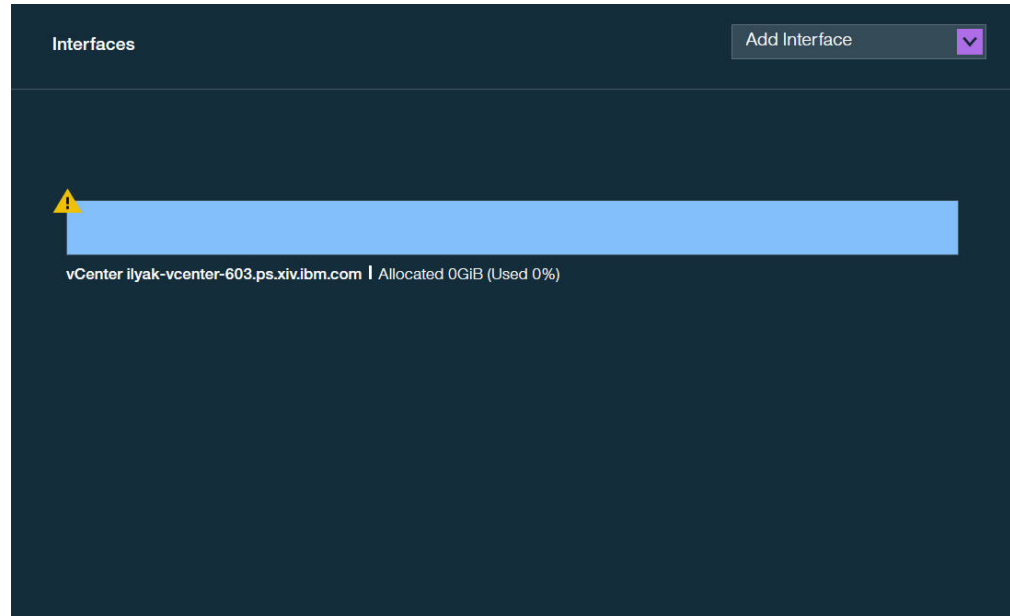
Figure 72. Interfaces pane
