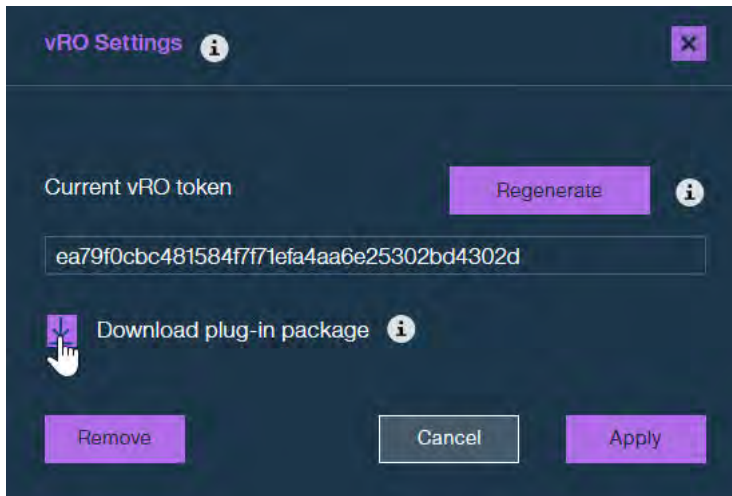
Figure 99. Download plug-in package button
