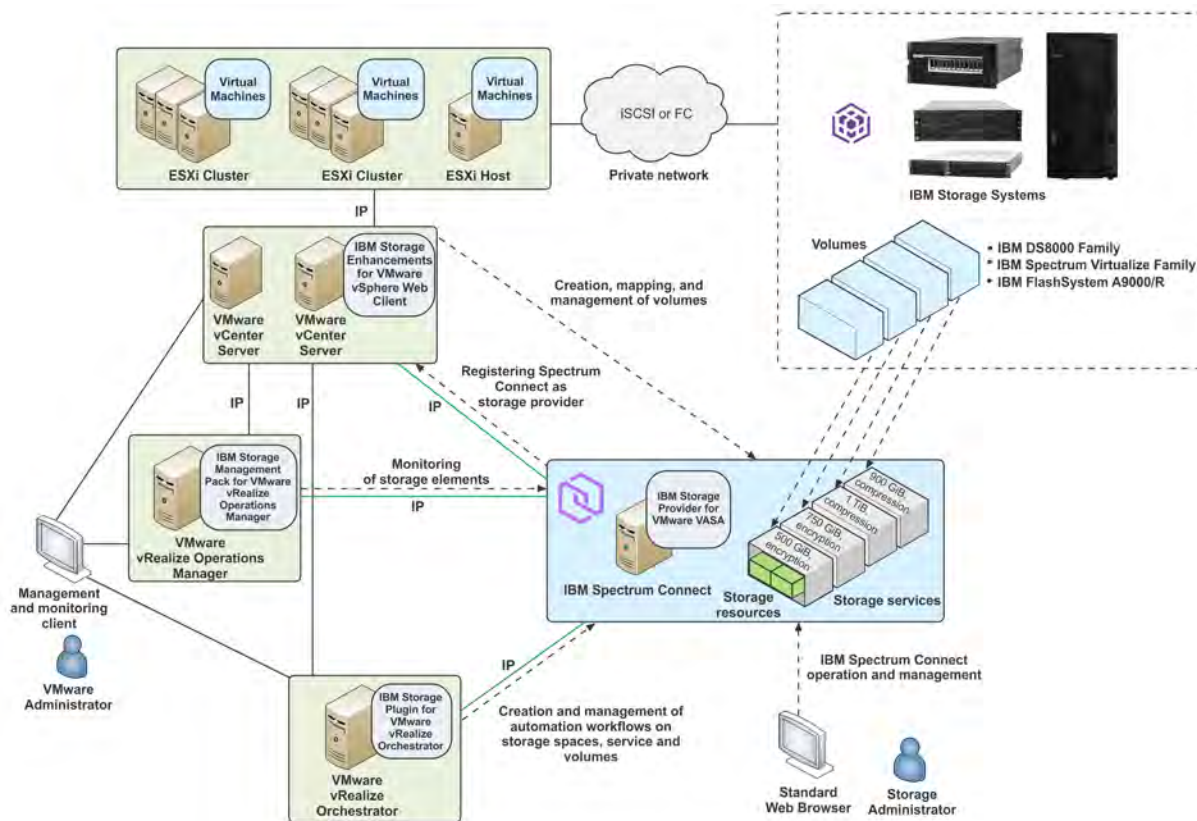
Figure 58. Integration of IBM storage systems with a VMware environment
