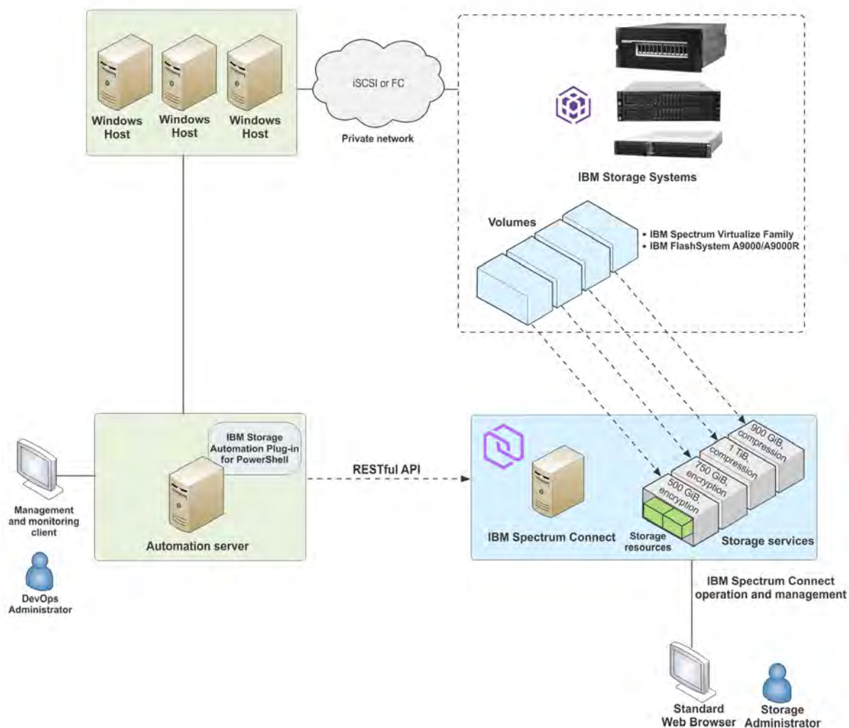
Figure 127. Integration of IBM storage systems in PowerShell environment
