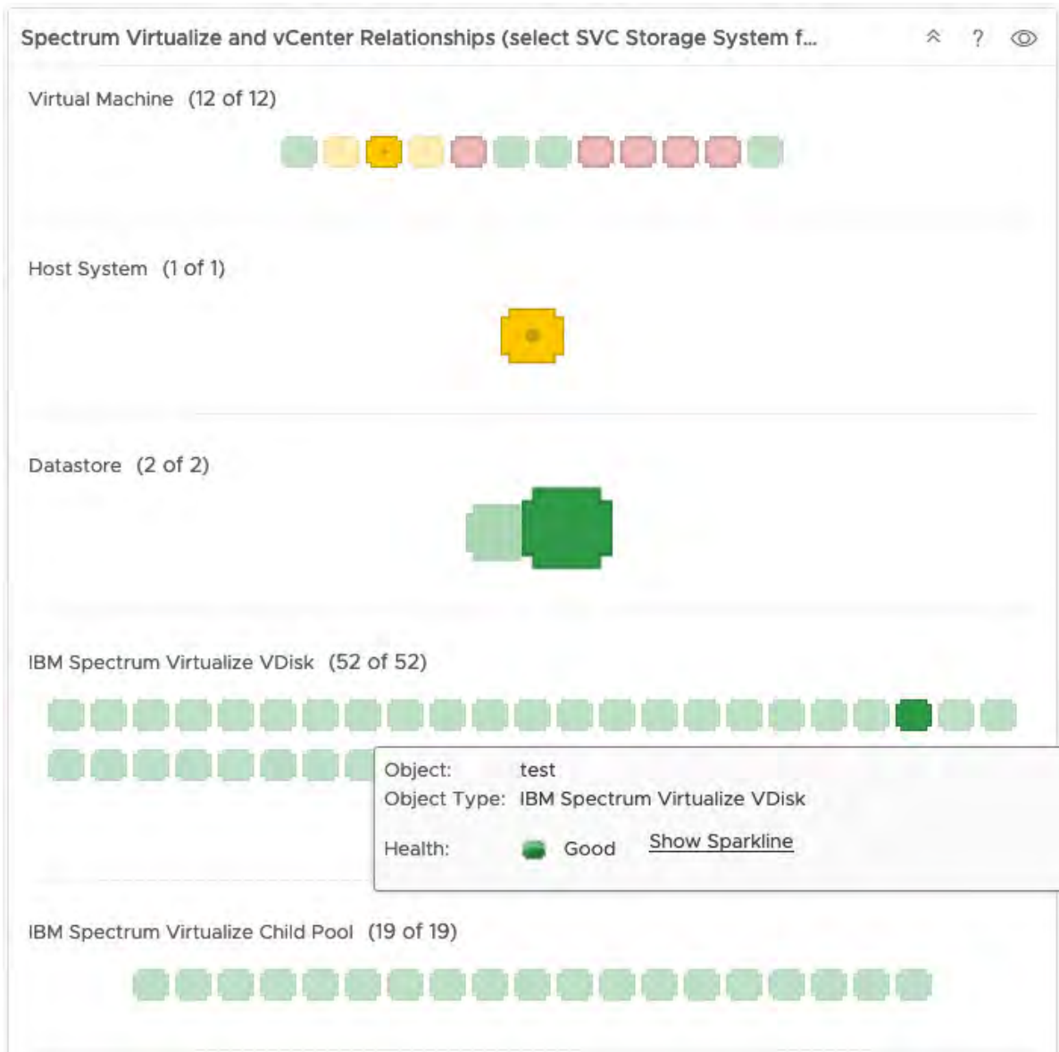
Figure 114. IBM Spectrum Virtualize vDisk health status
