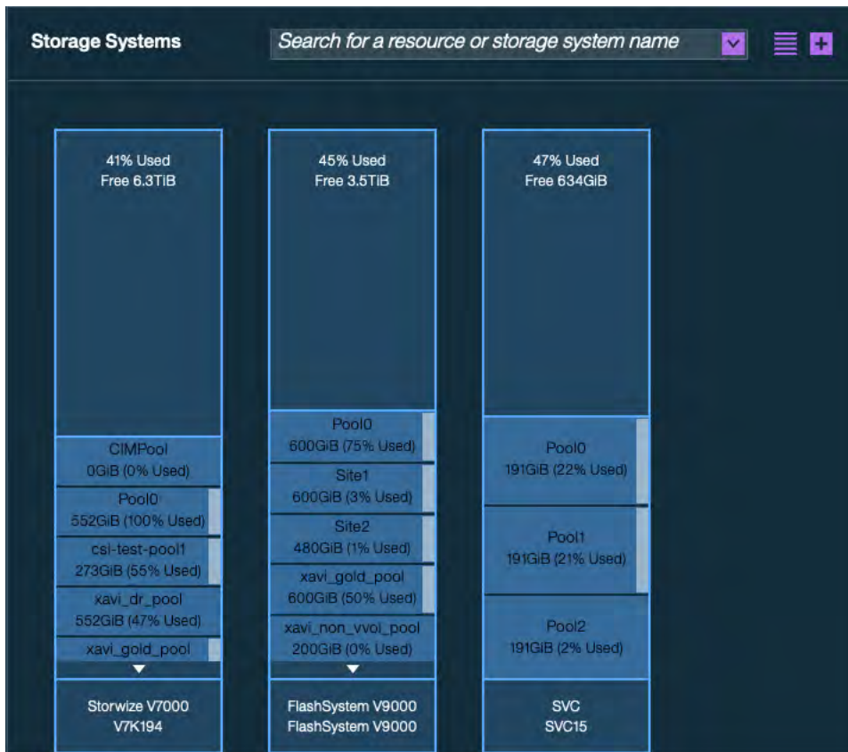
Figure 24. Storage Systems pane
