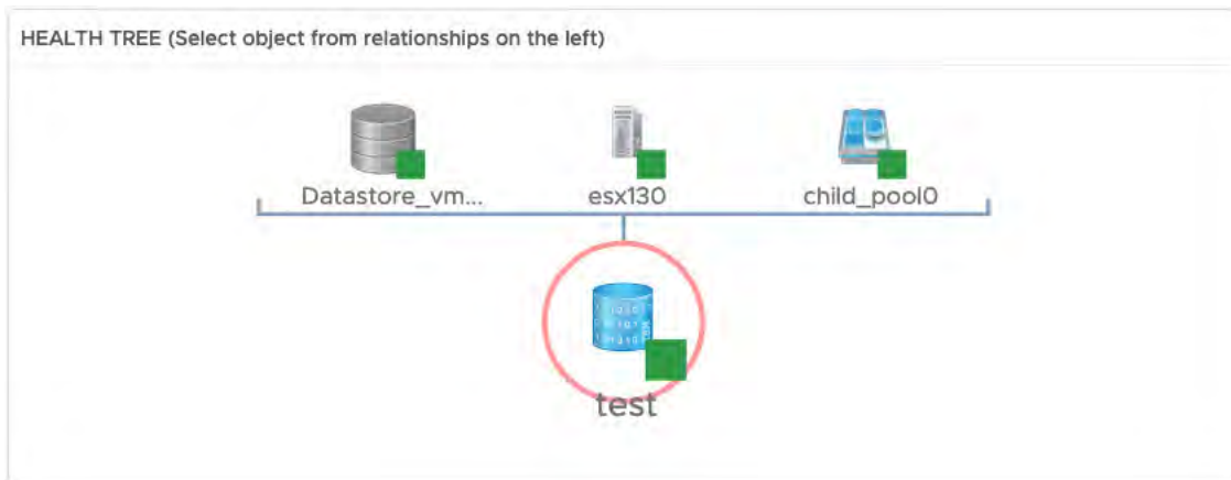
Figure 117. HEALTH TREE pane
