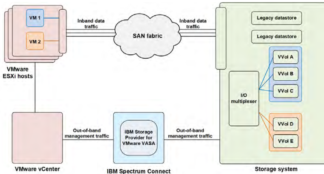
Figure 59. Using virtual volumes with IBM Spectrum Connect
