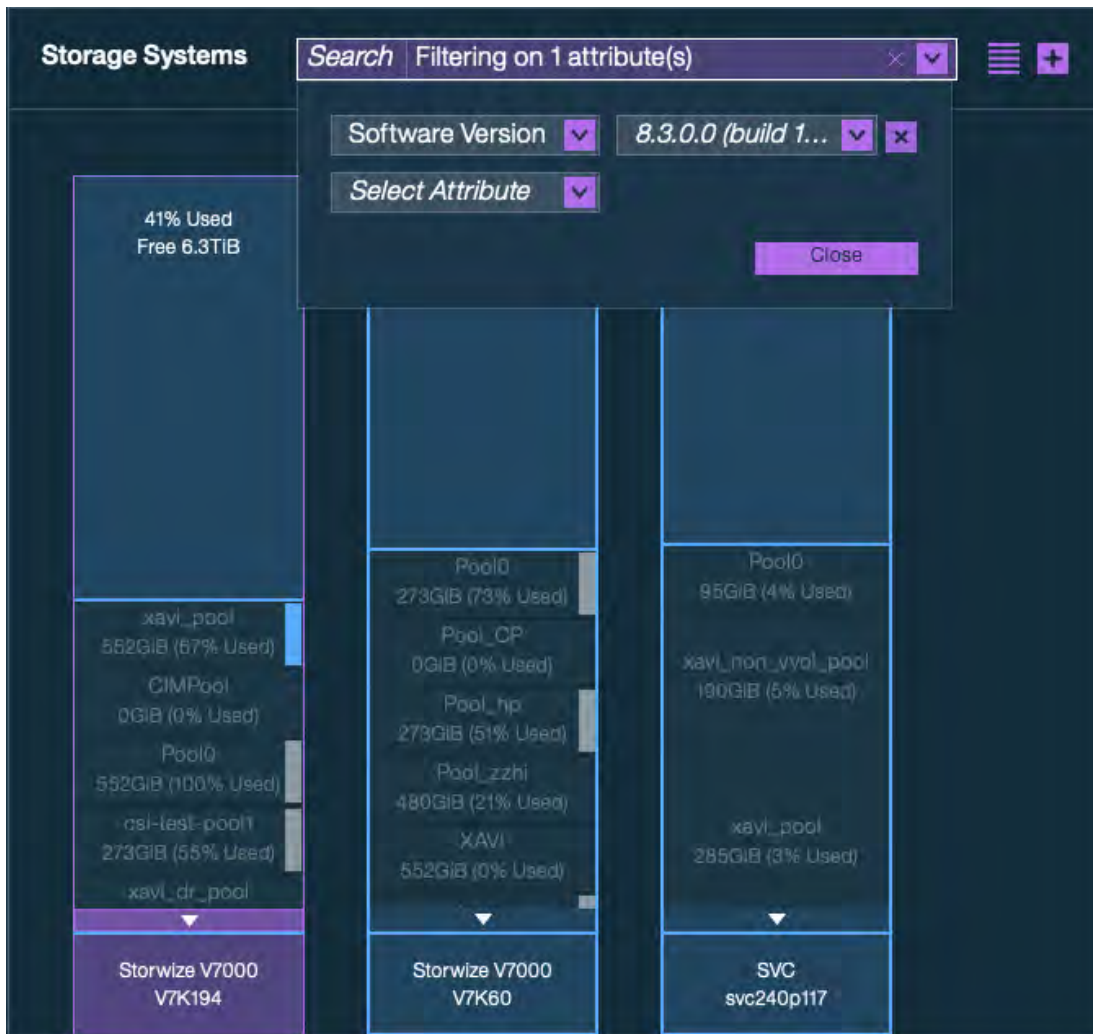
Figure 34. Storage Systems pane with storage elements filtered according to software version
