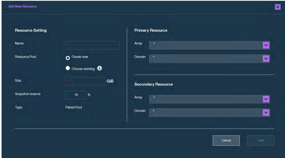
Figure 43. Add New Resource for replicated service dialog box, Create New option
