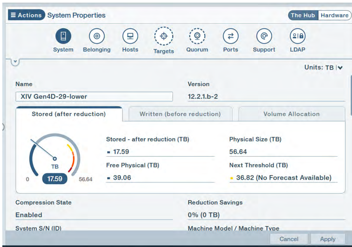
Figure 50. Hyper-Scale System Properties configuration view
