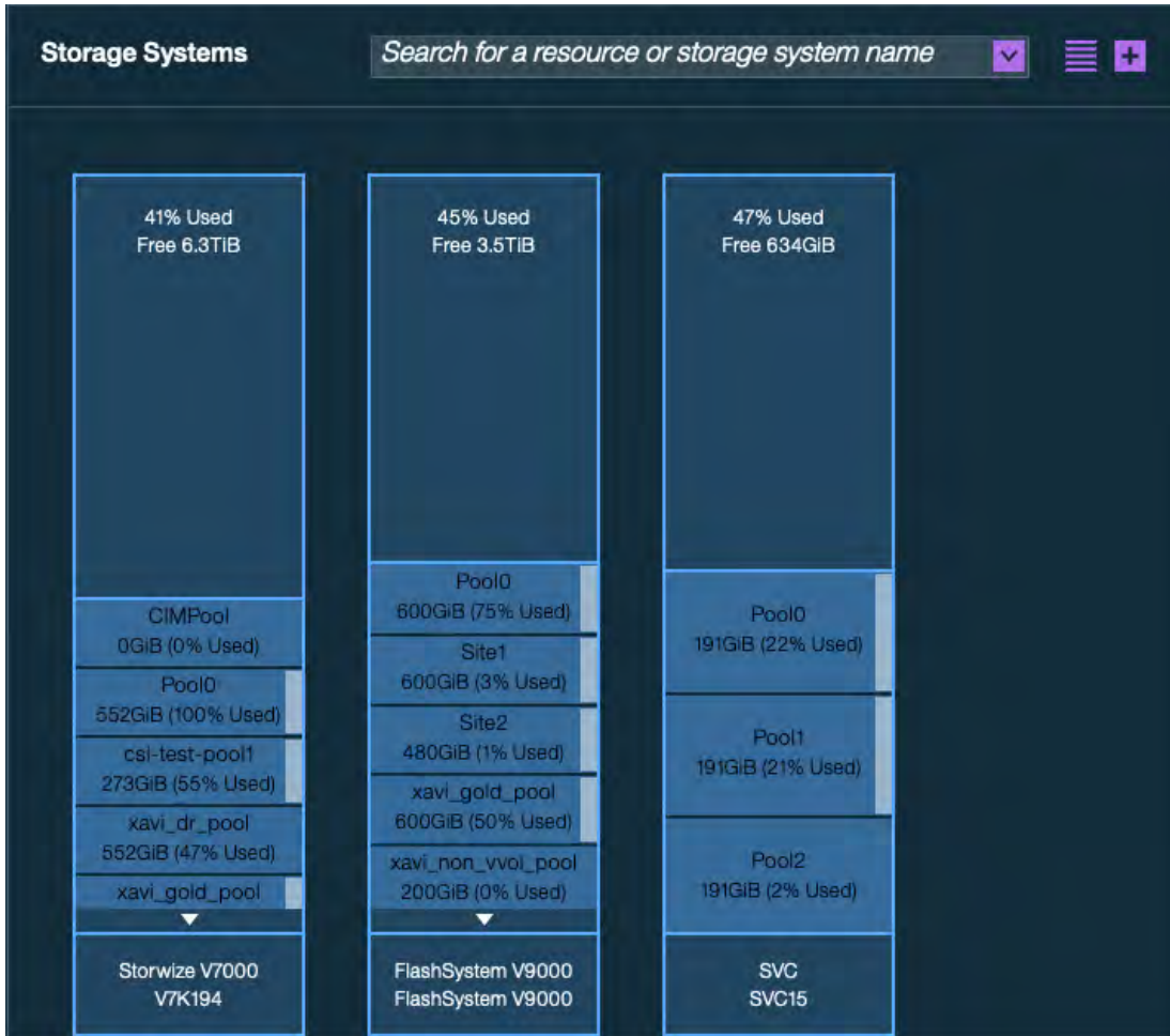
Figure 29. Storage Systems pane, bar view
